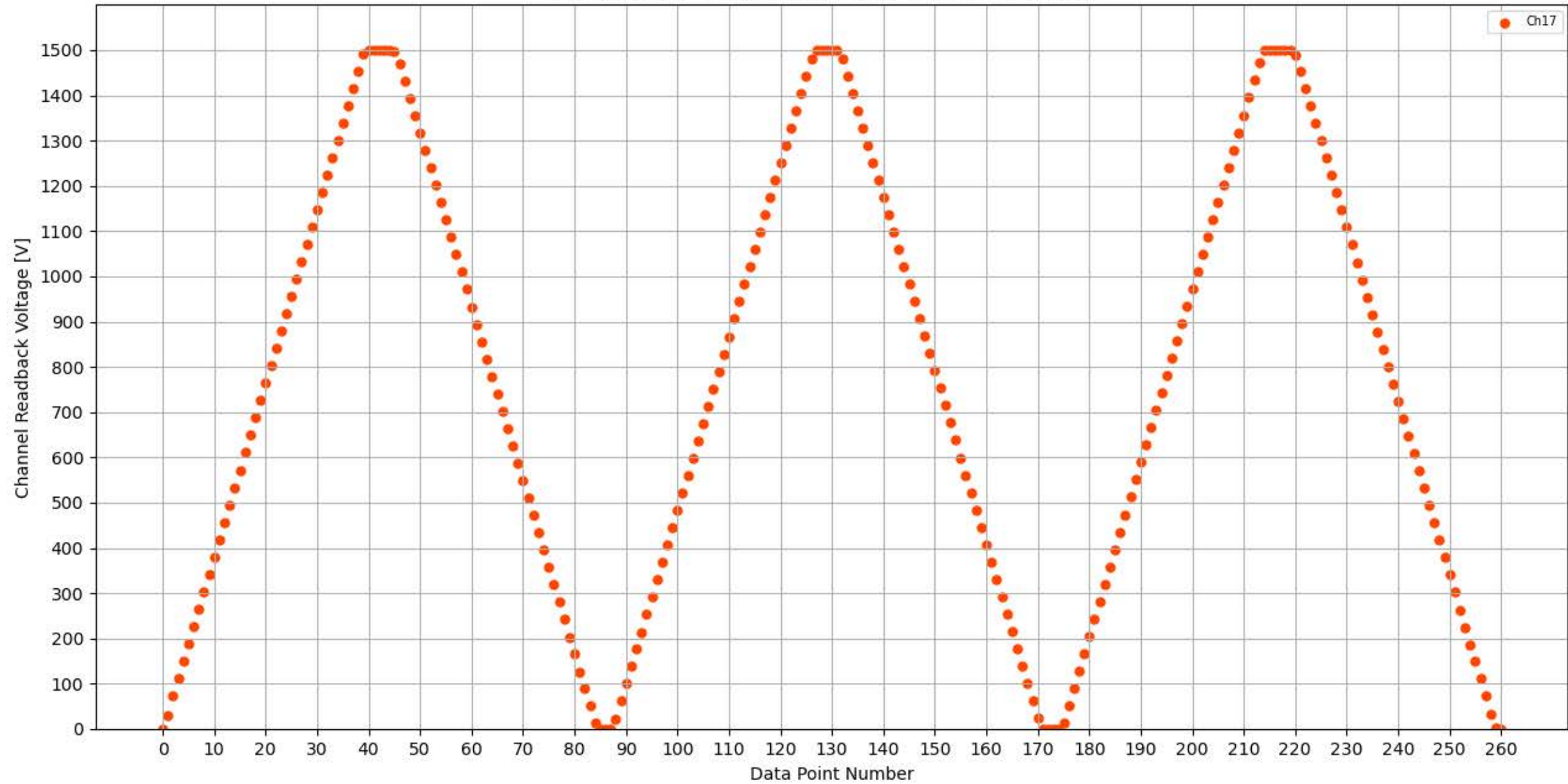
Voltage Ramp Test (Python) Bd #314, Slot #12, Ch #17
