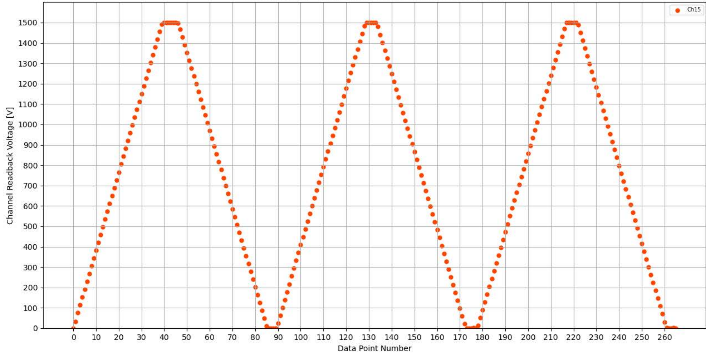
Voltage Ramp Test (Python) Bd #314, Slot #12, Ch #15
