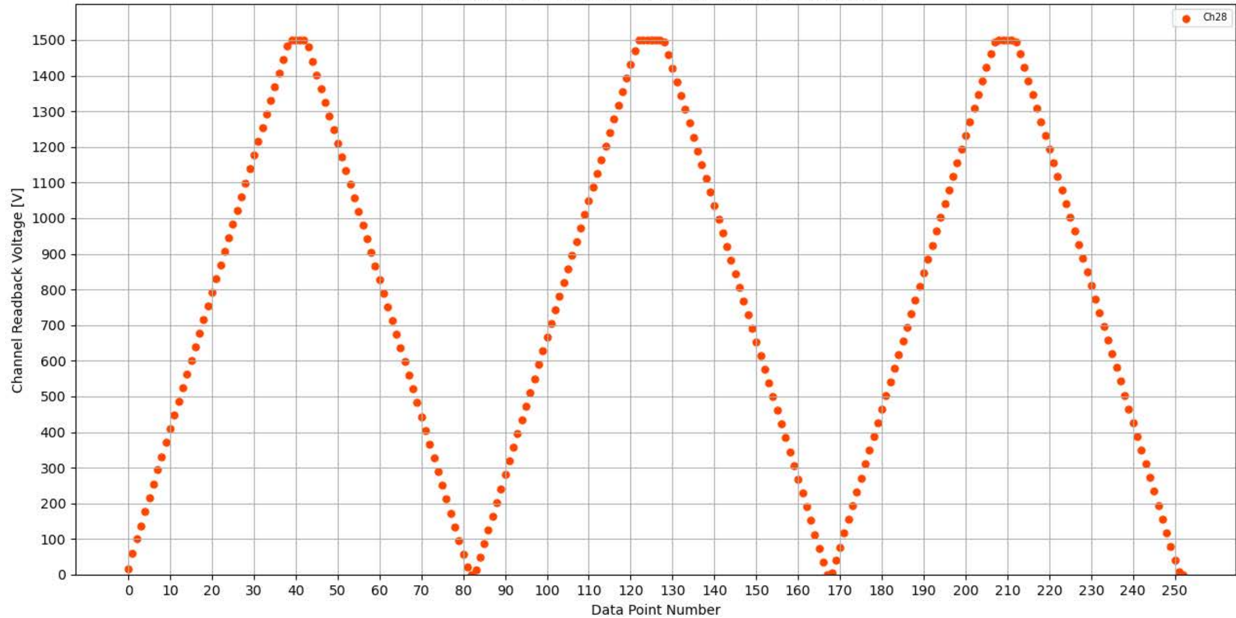
Voltage Ramp Test (Python) Bd #314, Slot #12, Ch #28
