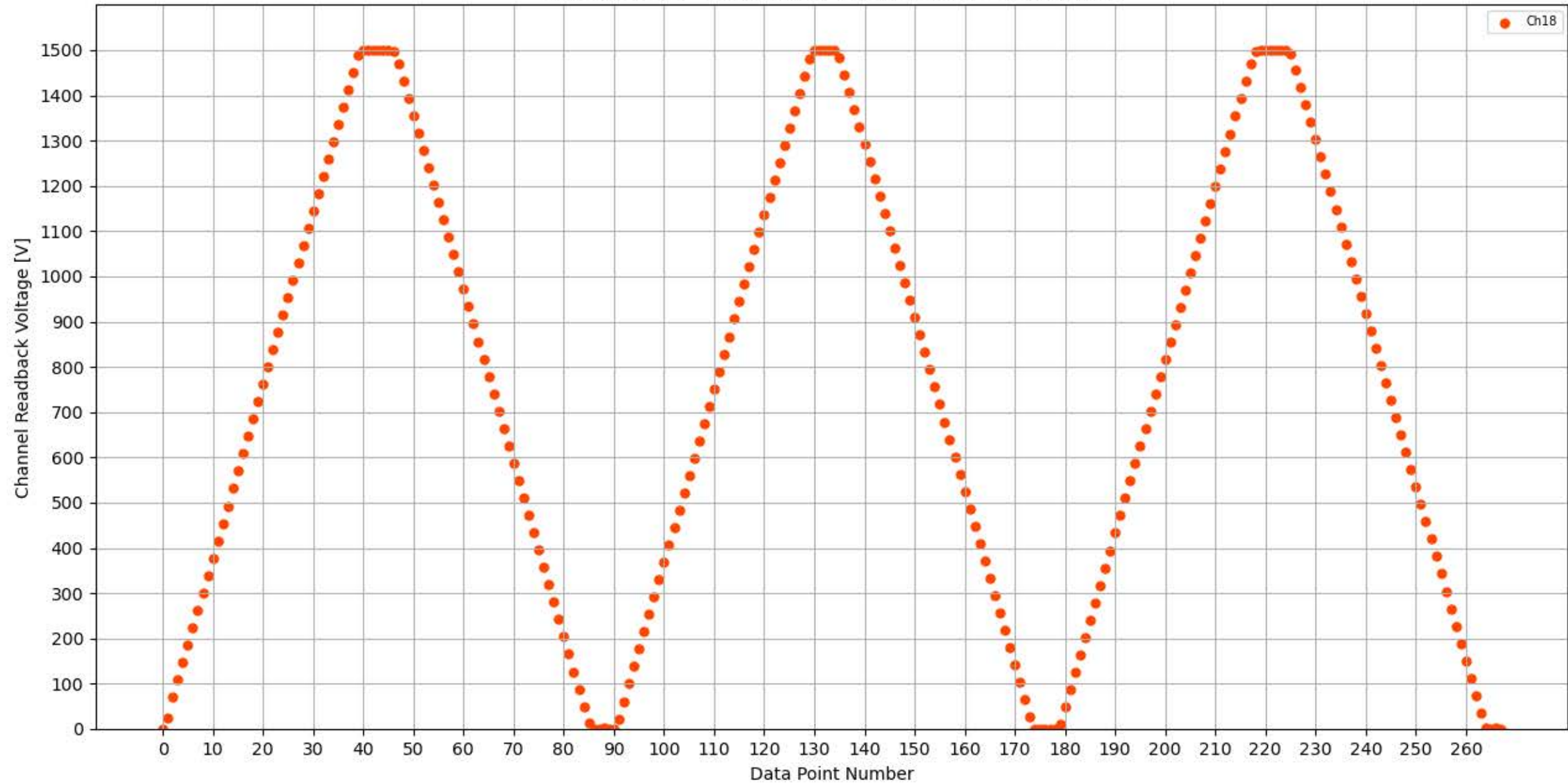
Voltage Ramp Test (Python) Bd #314, Slot #12, Ch #18
