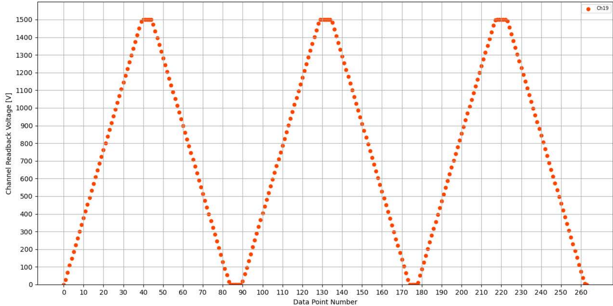
Voltage Ramp Test (Python) Bd #314, Slot #12, Ch #19
