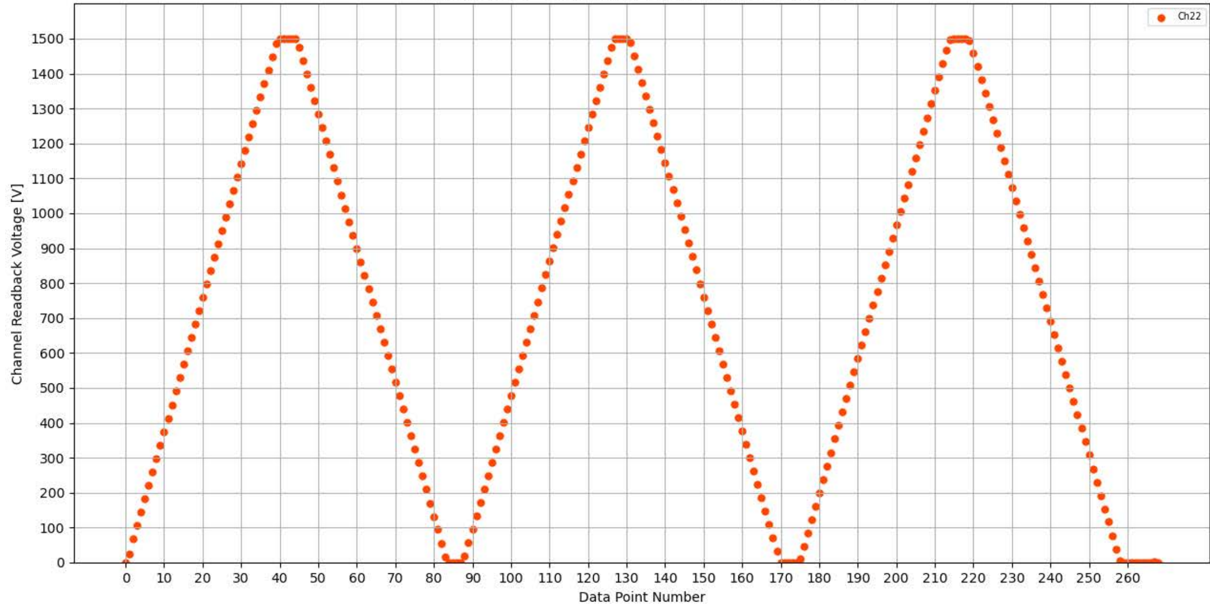
Voltage Ramp Test (Python) Bd #314, Slot #12, Ch #22
