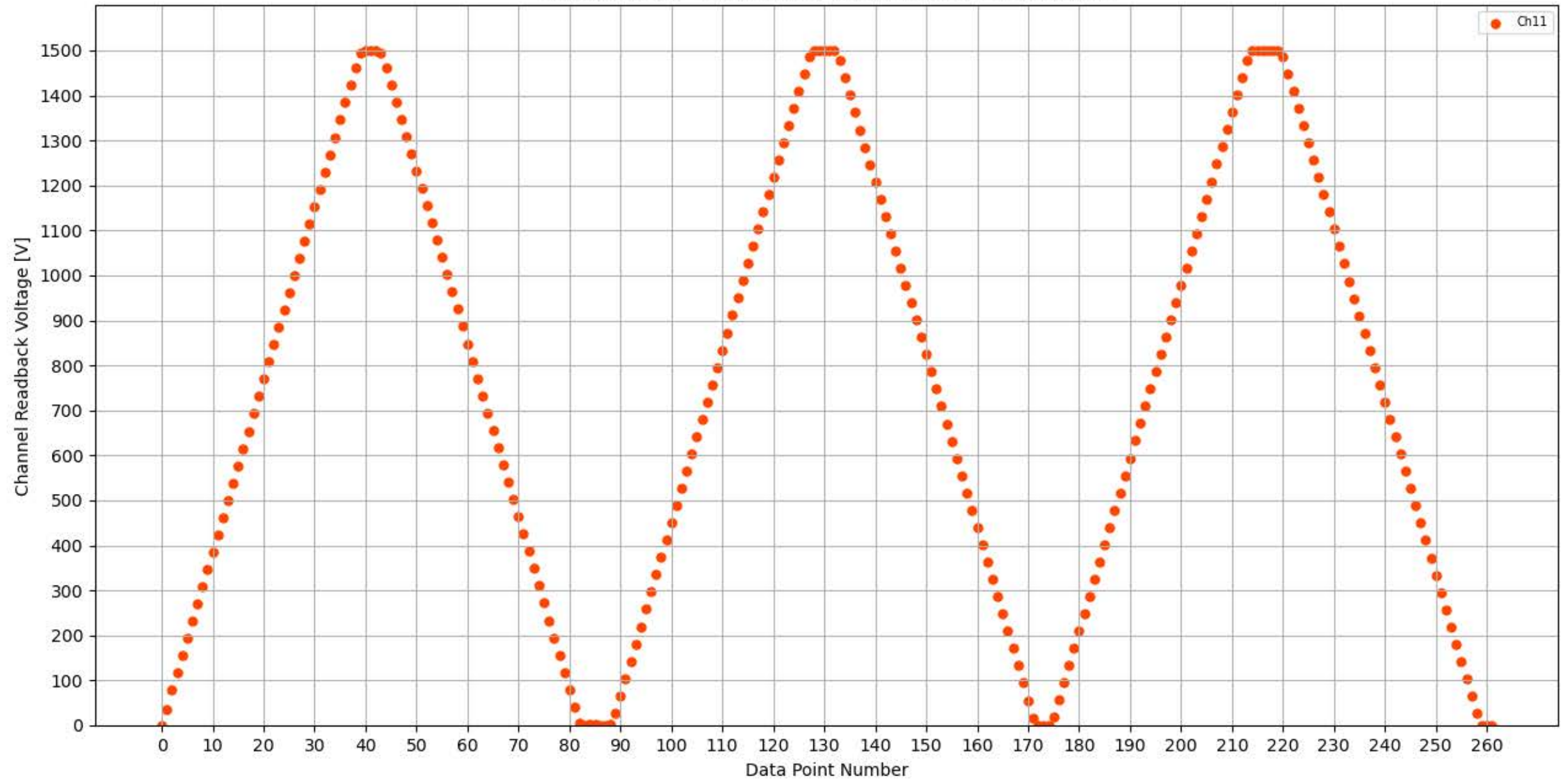
Voltage Ramp Test (Python) Bd #314, Slot #12, Ch #11
