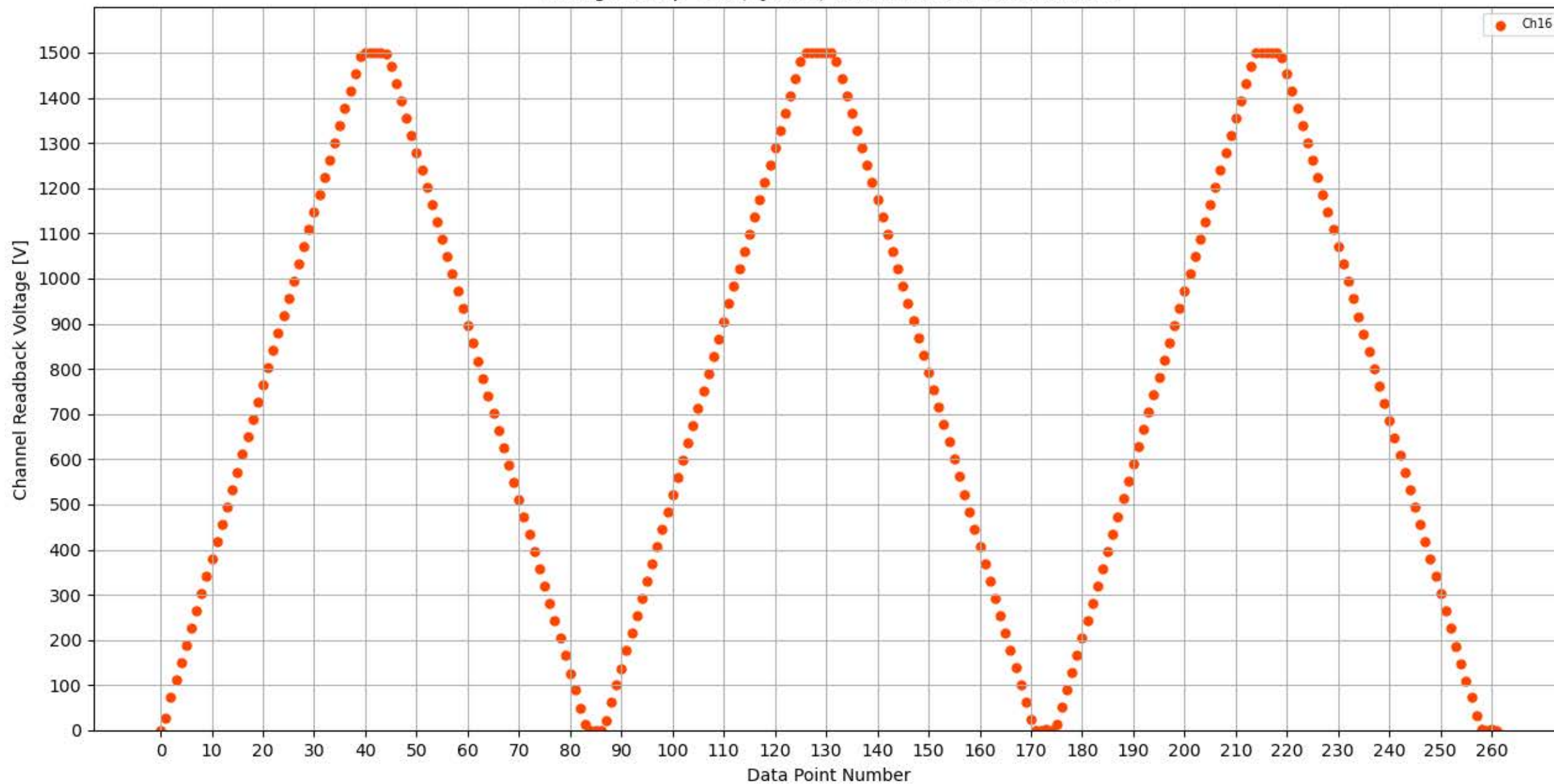
Voltage Ramp Test (Python) Bd #314, Slot #12, Ch #16
