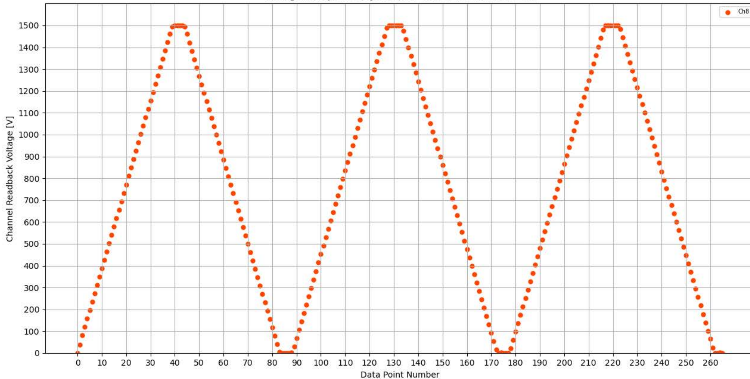
Voltage Ramp Test (Python) Bd #314, Slot #12, Ch #8
