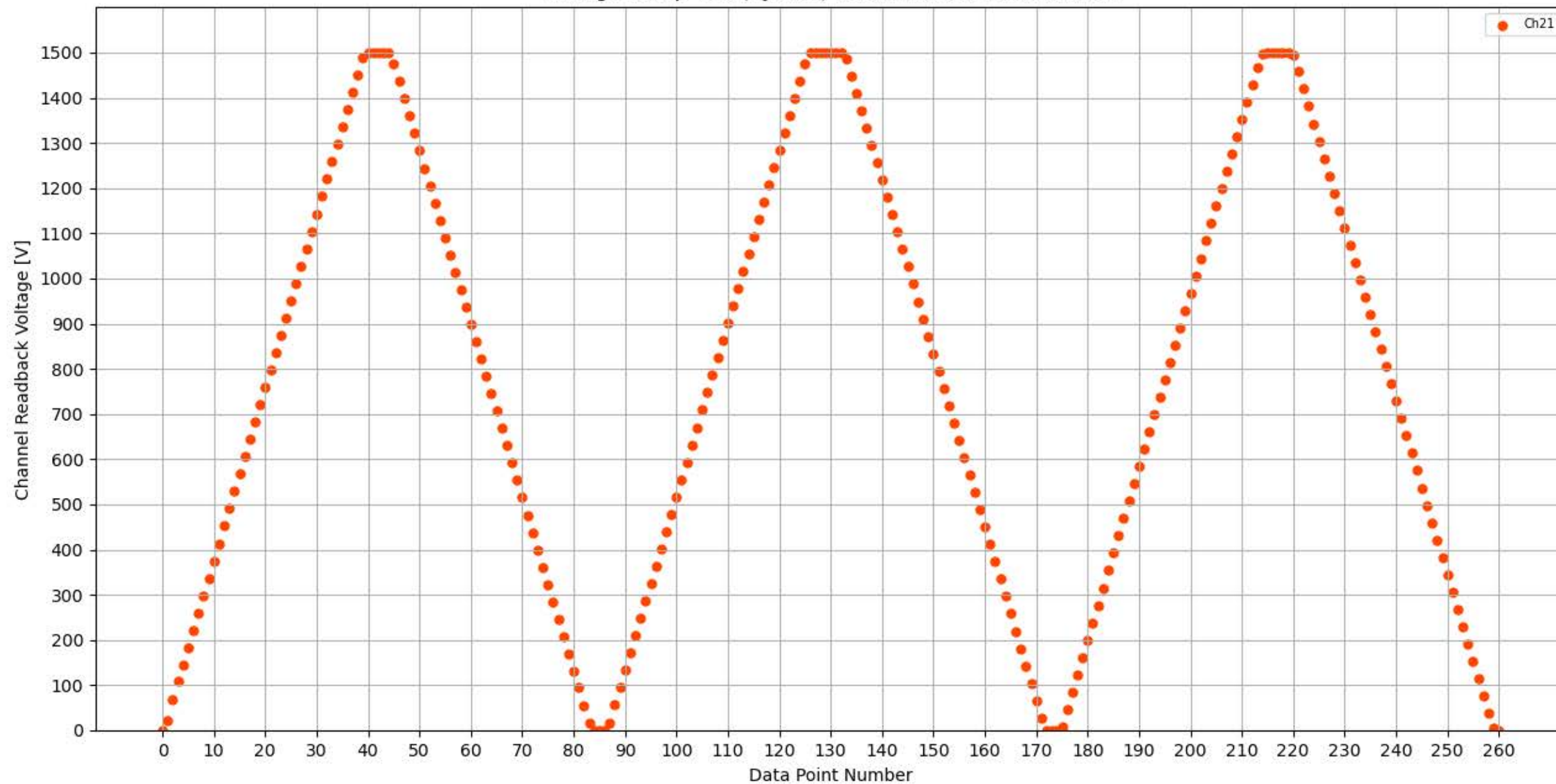
Voltage Ramp Test (Python) Bd #314, Slot #12, Ch #21
