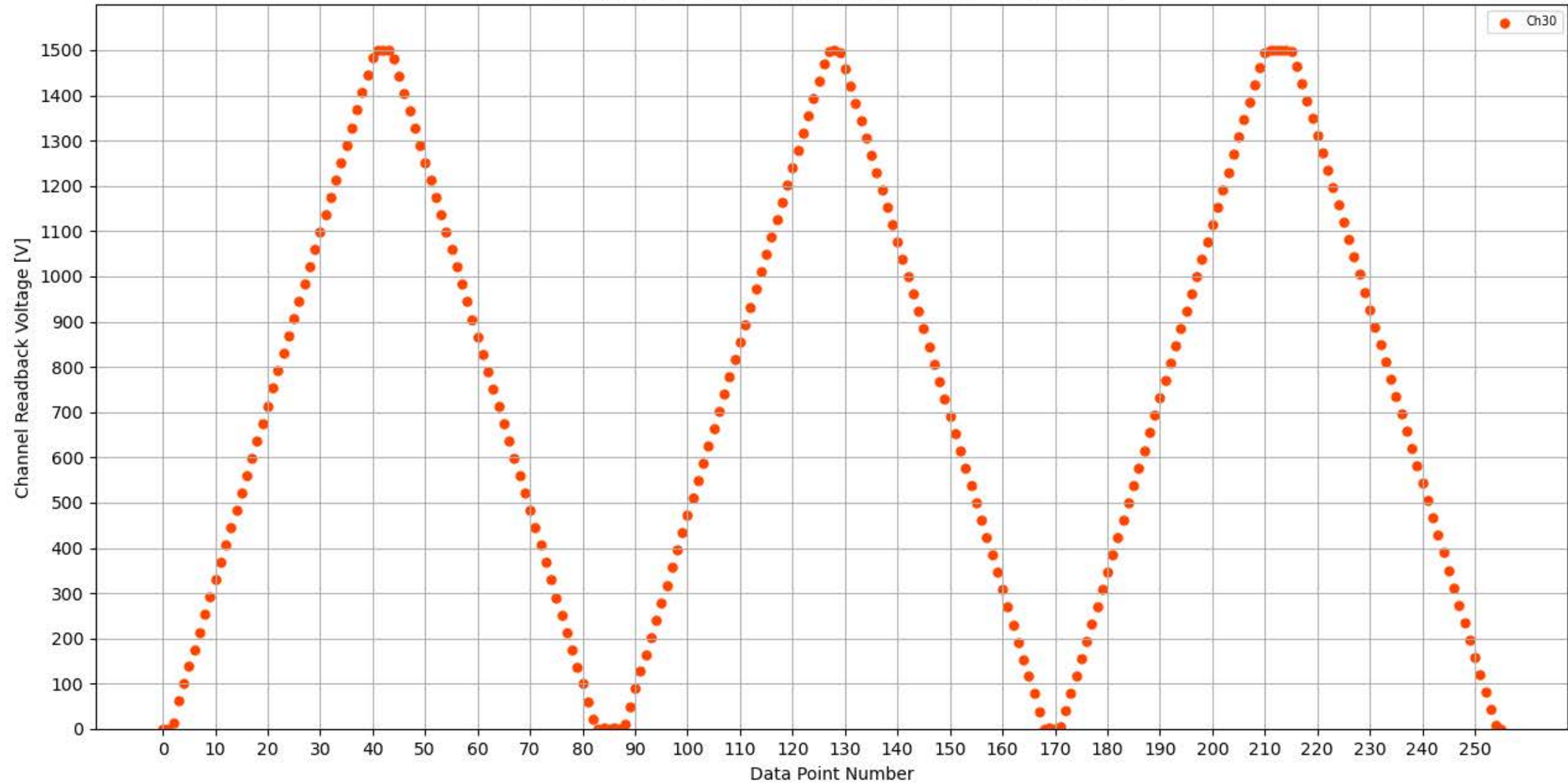
Voltage Ramp Test (Python) Bd #314, Slot #12, Ch #30
