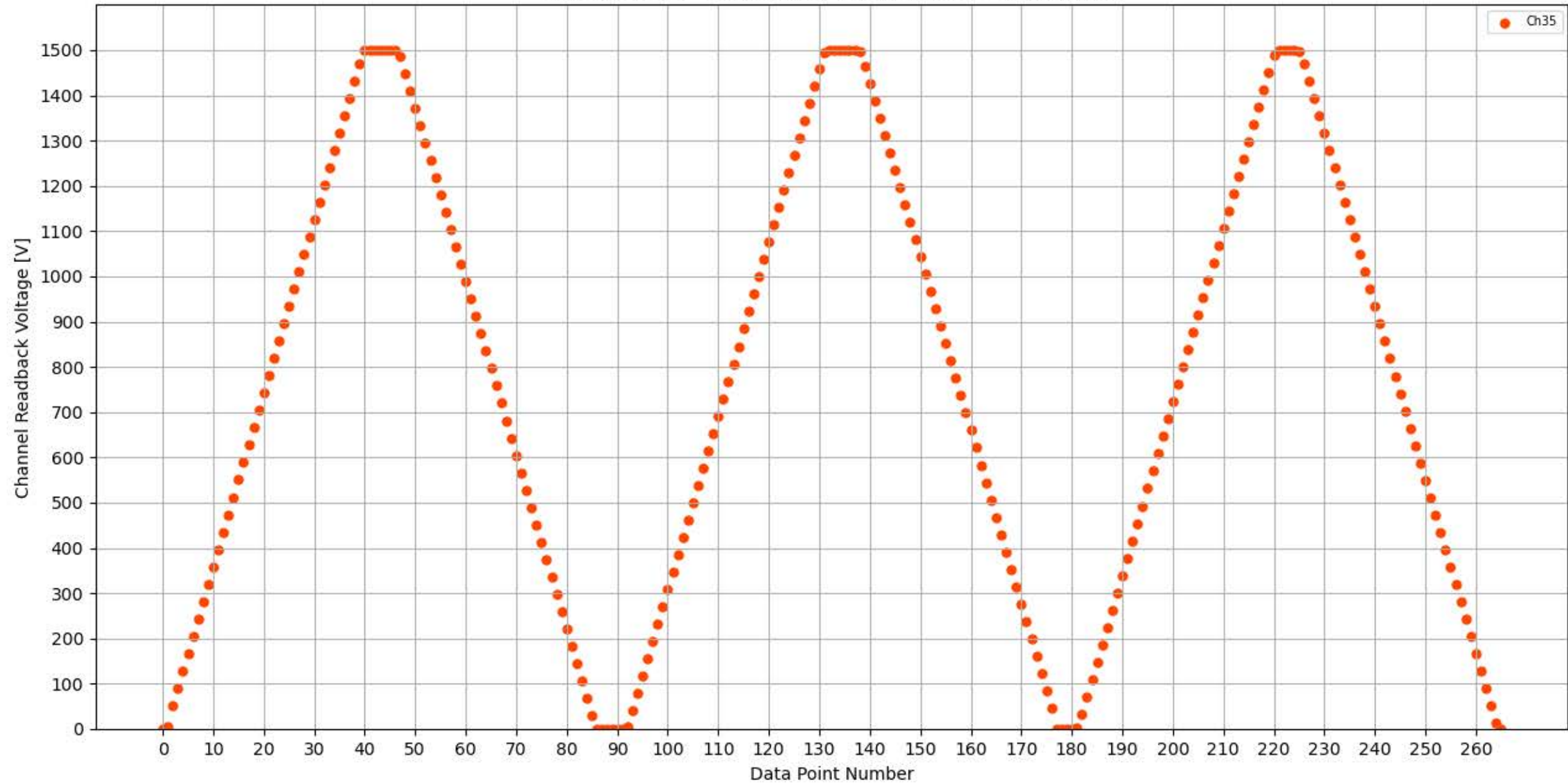
Voltage Ramp Test (Python) Bd #314, Slot #12, Ch #35
