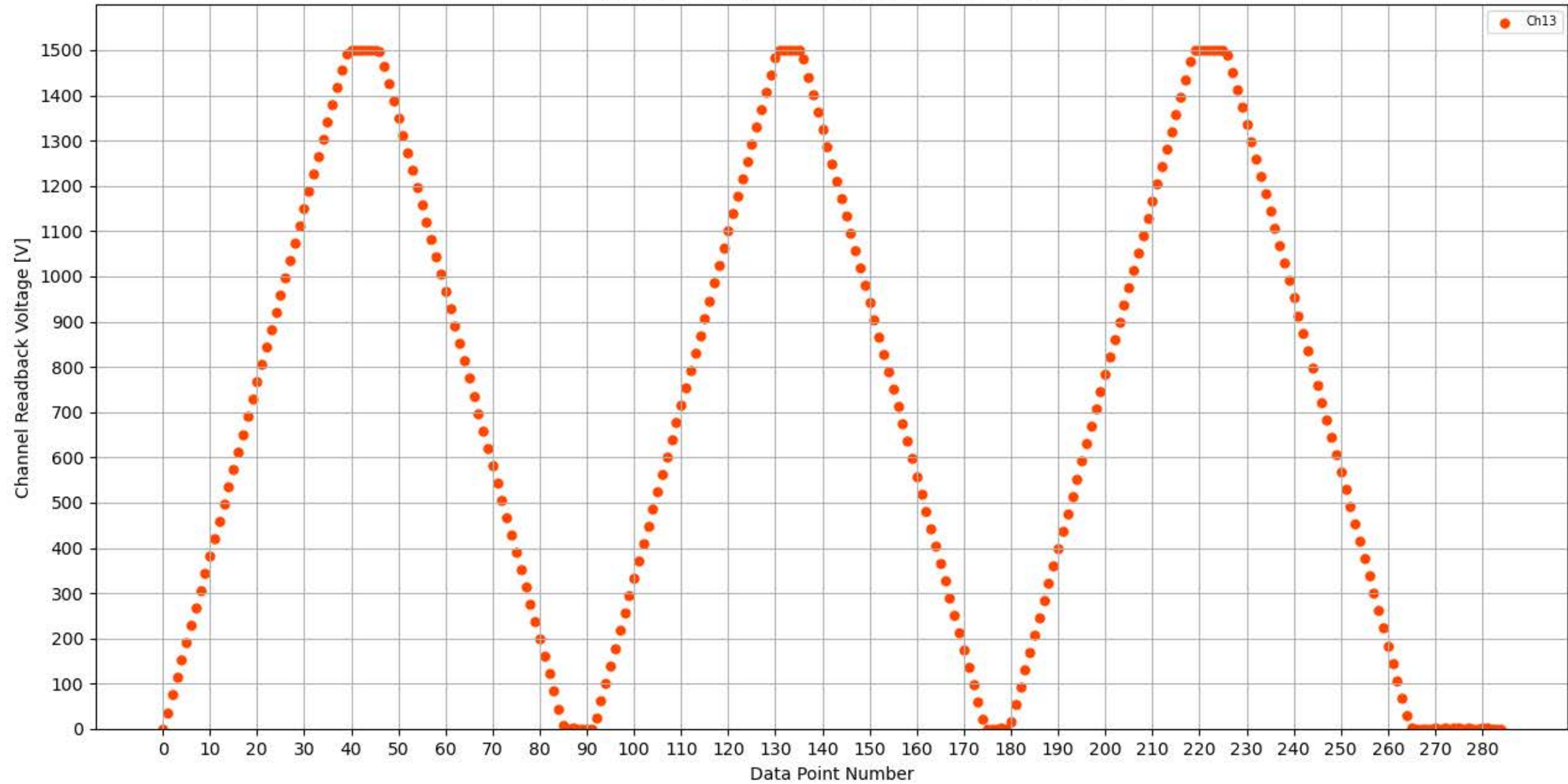
Voltage Ramp Test (Python) Bd #314, Slot #12, Ch #13
