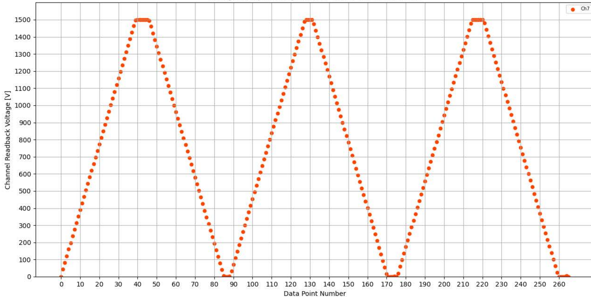
Voltage Ramp Test (Python) Bd #314, Slot #12, Ch #7
