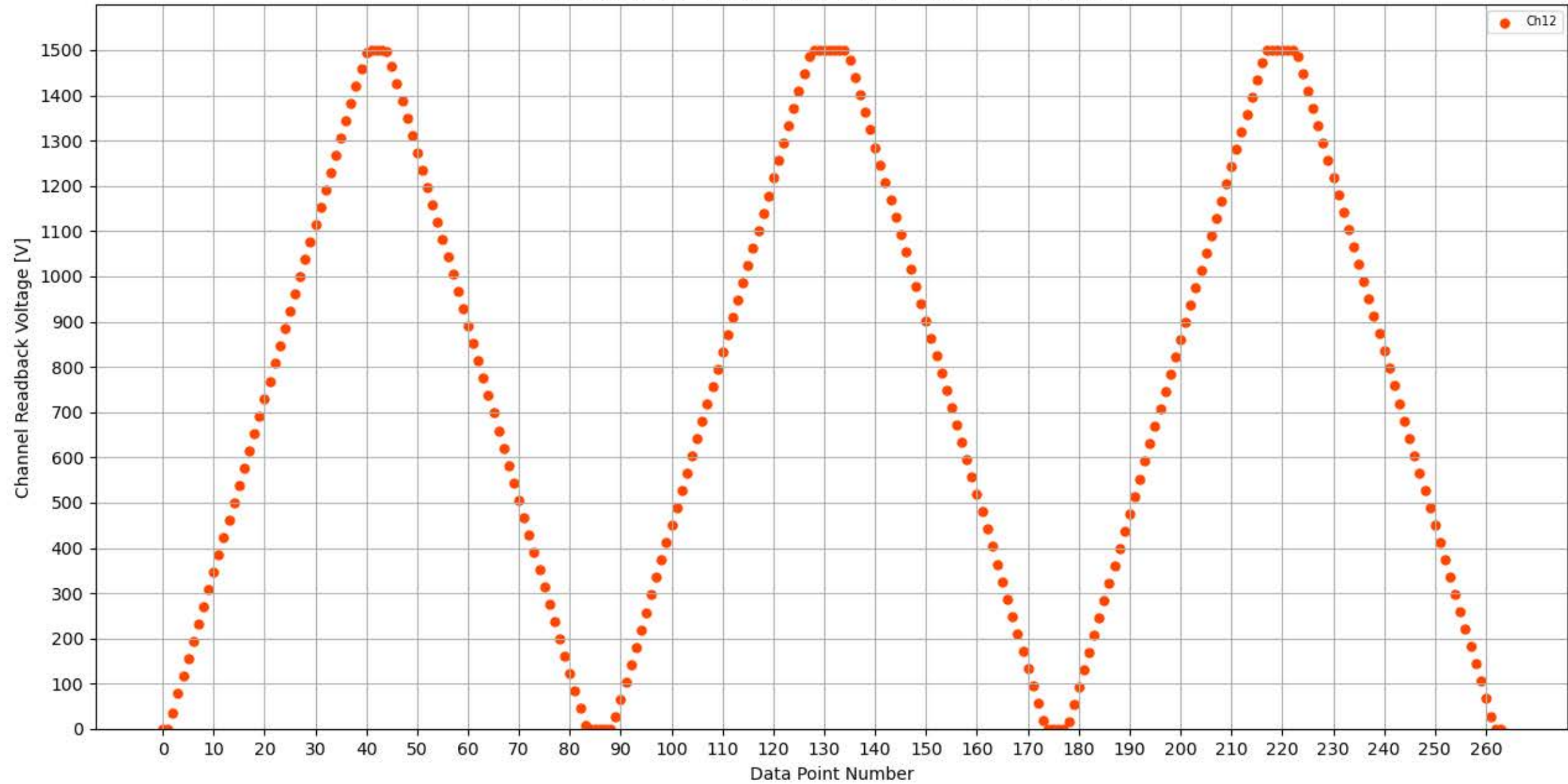
Voltage Ramp Test (Python) Bd #314, Slot #12, Ch #12
