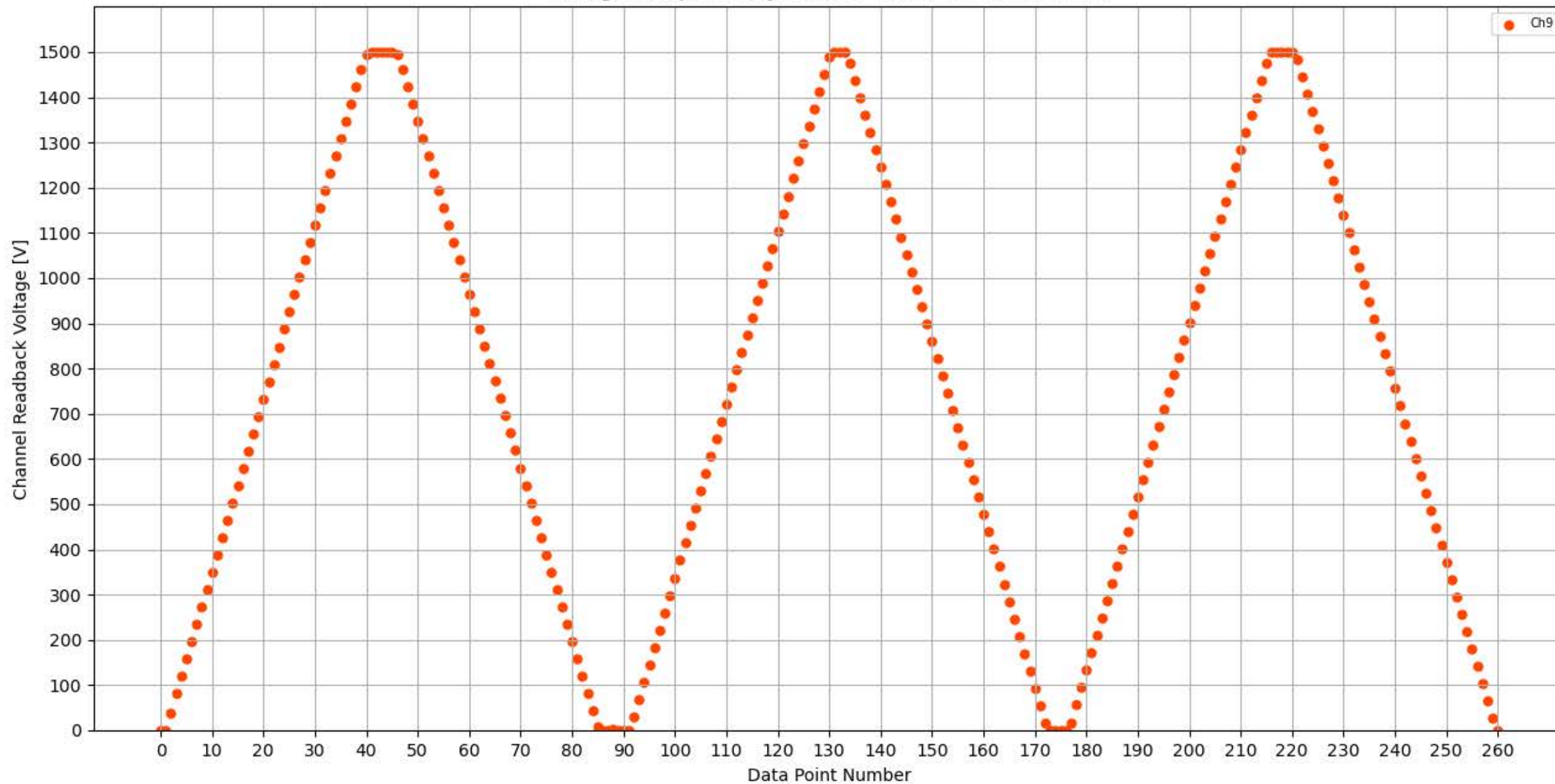
Voltage Ramp Test (Python) Bd #314, Slot #12, Ch #9
