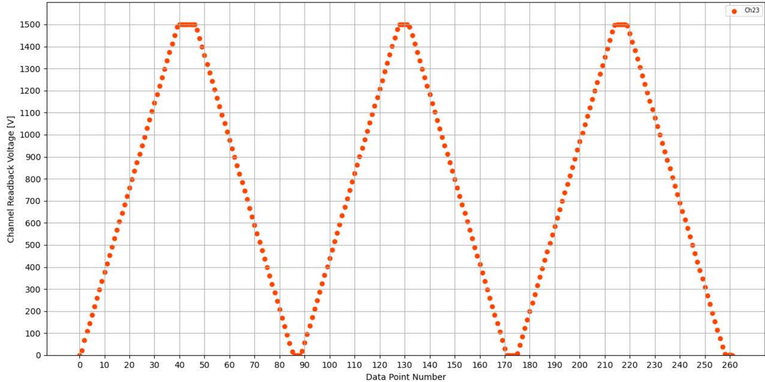
Voltage Ramp Test (Python) Bd #314, Slot #12, Ch #23
