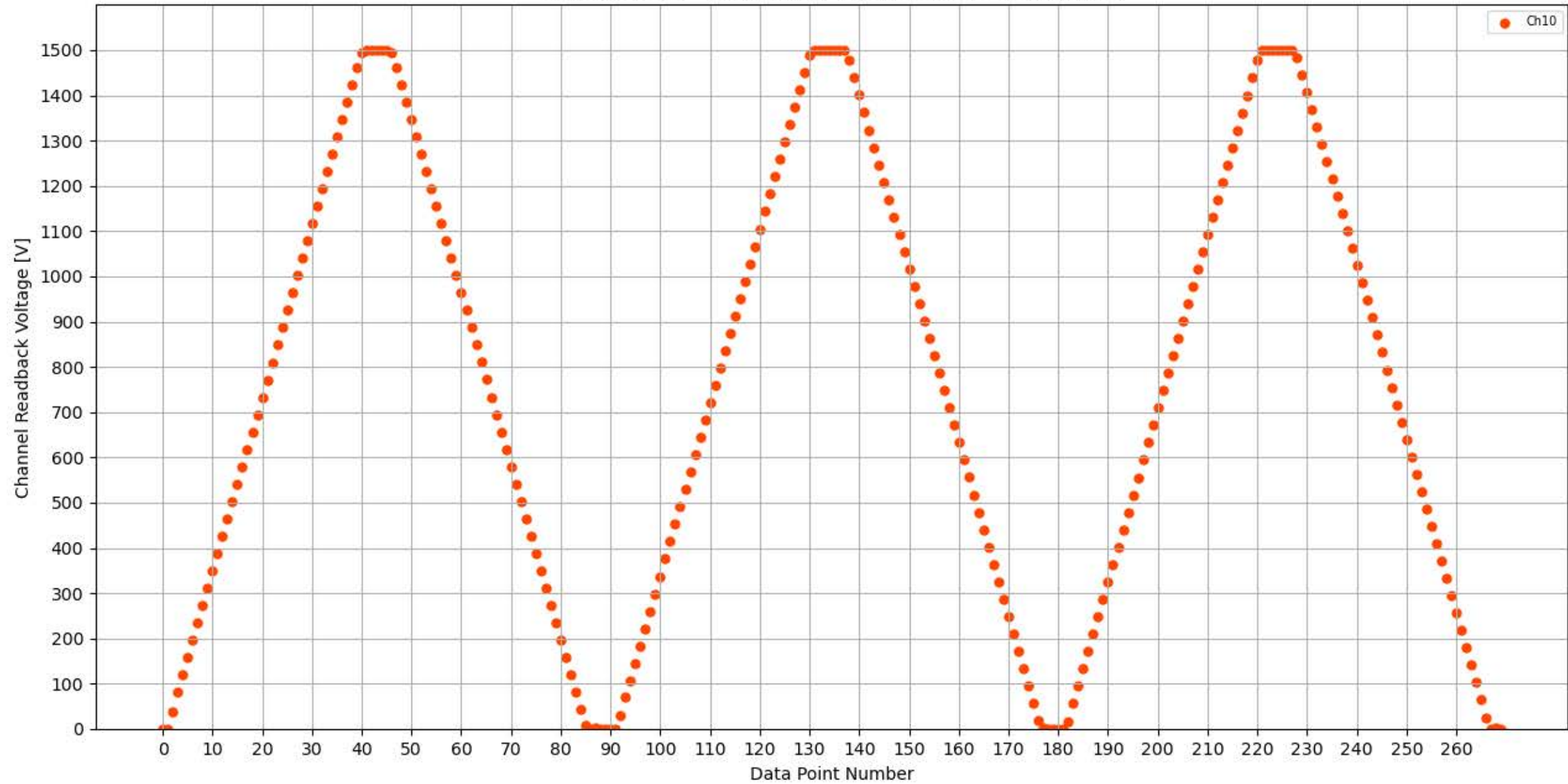
Voltage Ramp Test (Python) Bd #314, Slot #12, Ch #10
