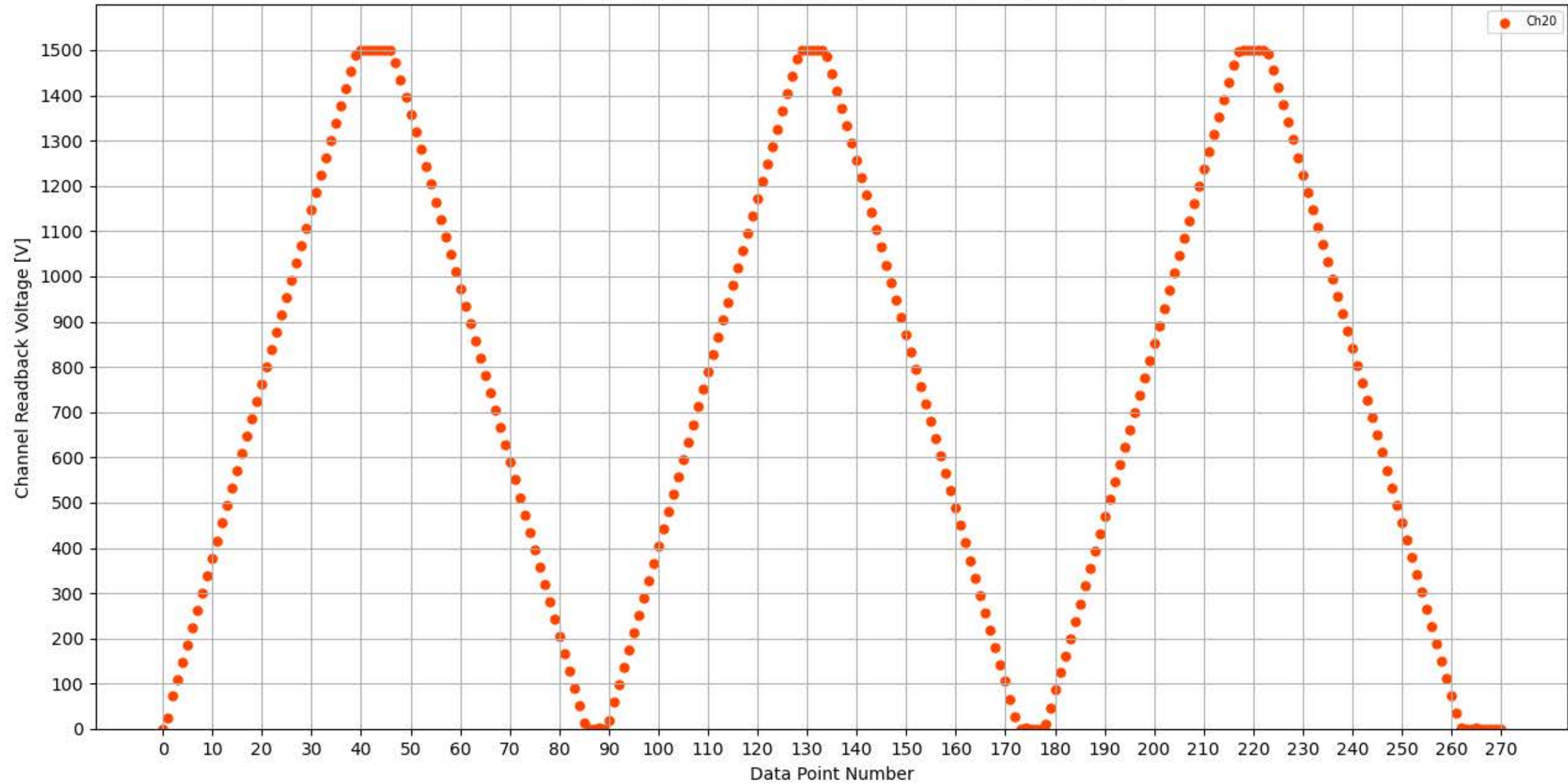
Voltage Ramp Test (Python) Bd #314, Slot #12, Ch #20
