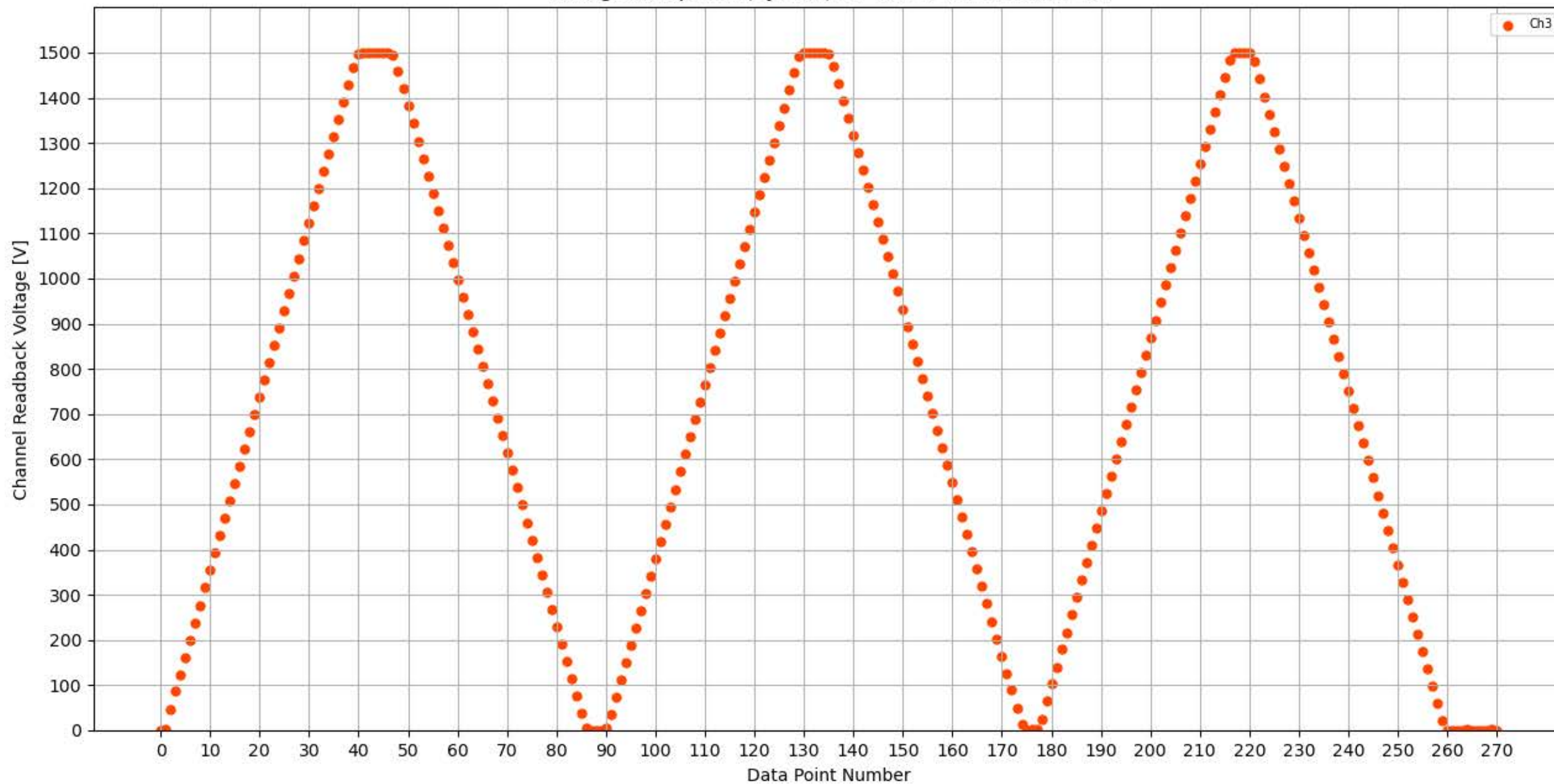
Voltage Ramp Test (Python) Bd #314, Slot #12, Ch #3
