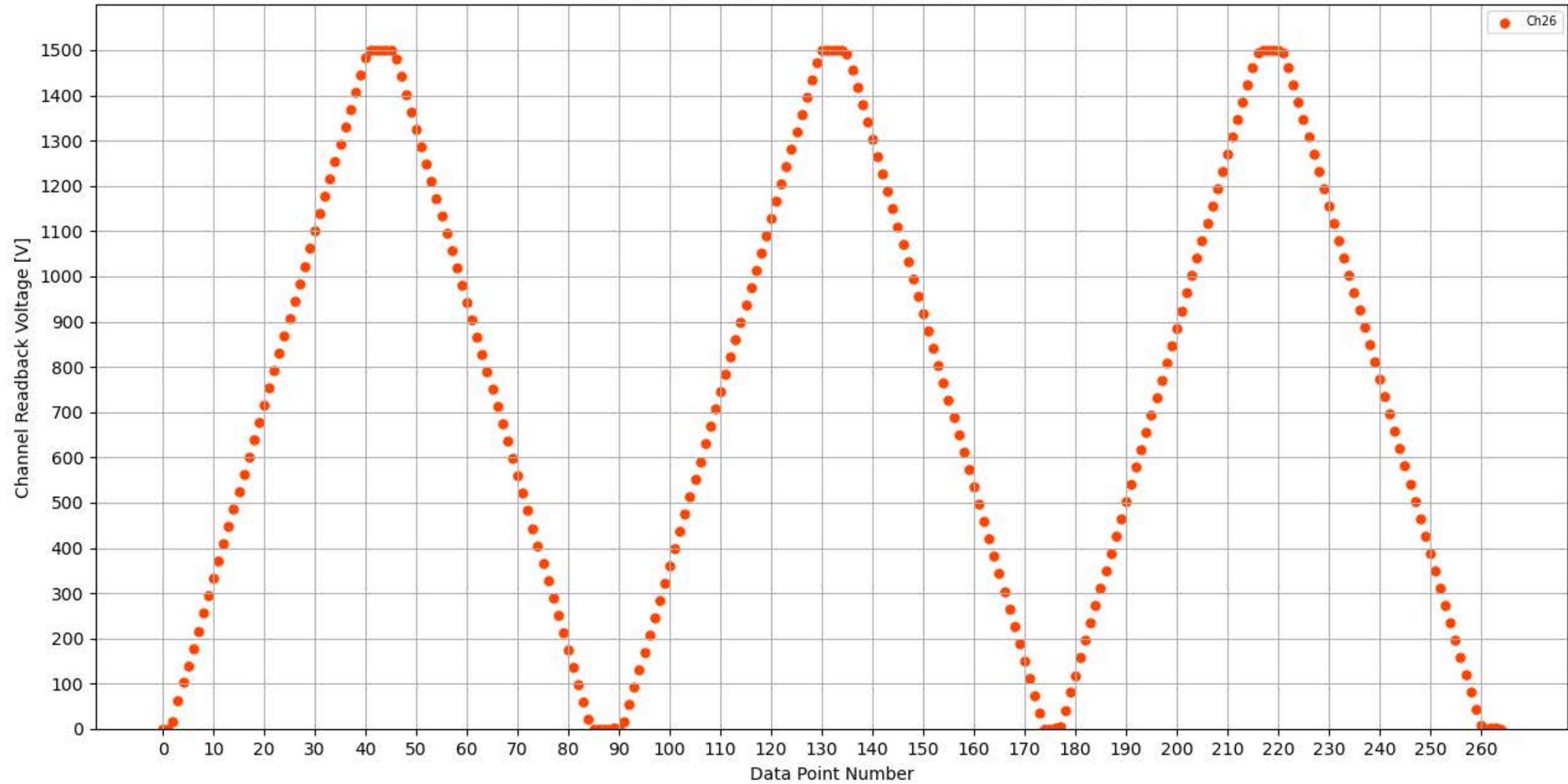
Voltage Ramp Test (Python) Bd #314, Slot #12, Ch #26
