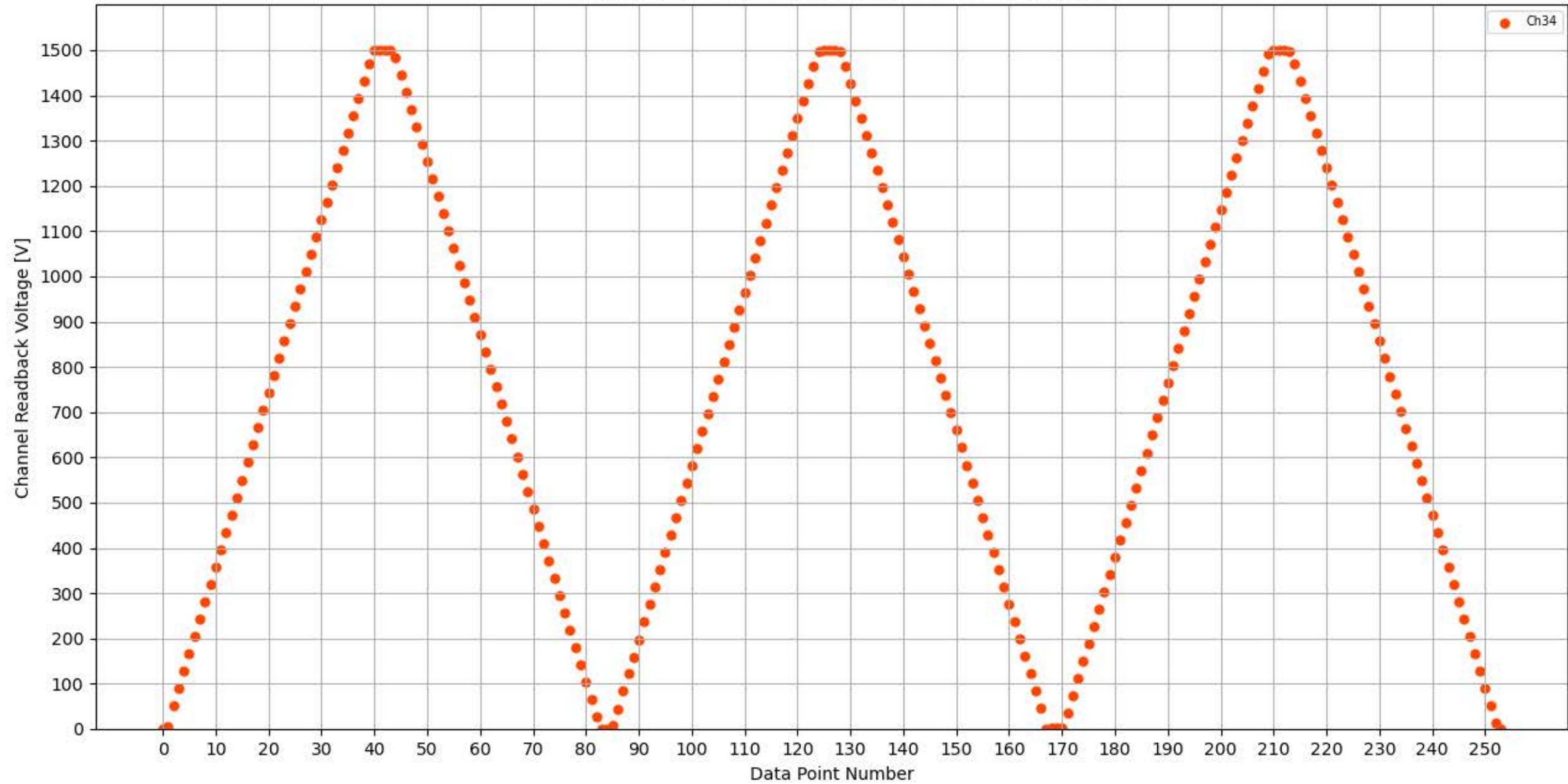
Voltage Ramp Test (Python) Bd #314, Slot #12, Ch #34
