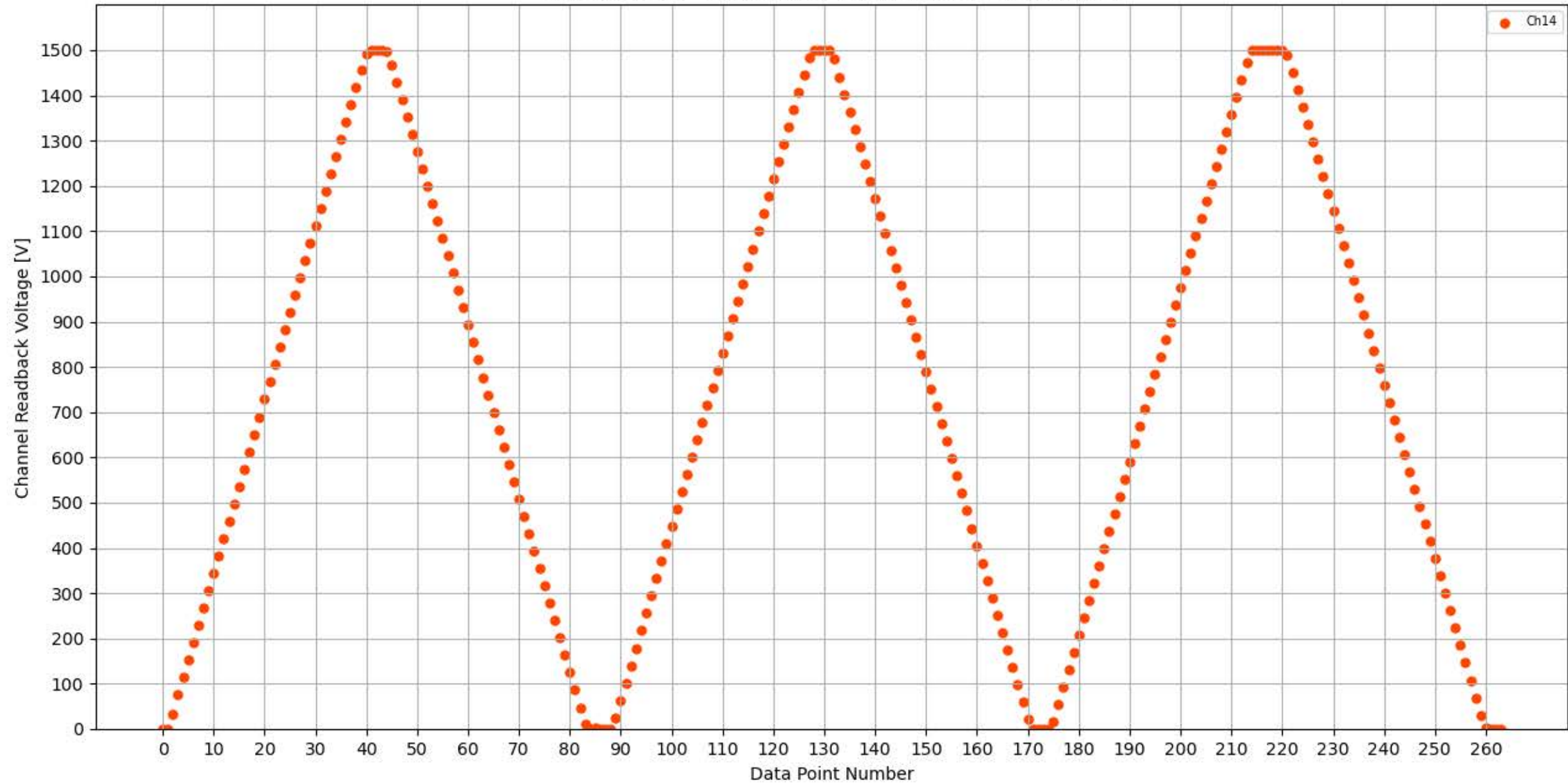
Voltage Ramp Test (Python) Bd #314, Slot #12, Ch #14
