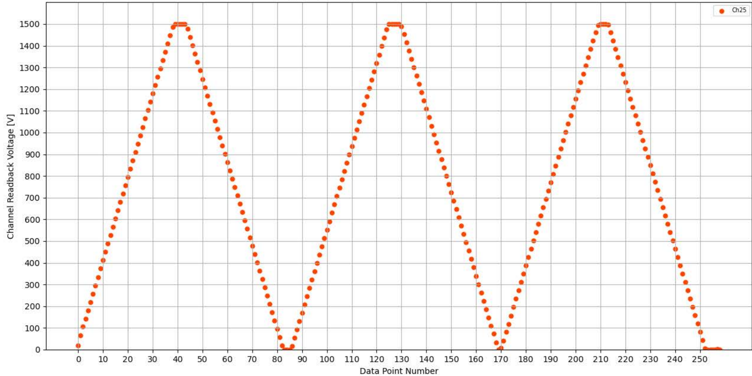
Voltage Ramp Test (Python) Bd #314, Slot #12, Ch #25
